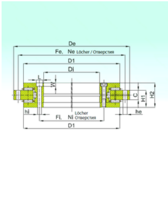
YRT 580 Bearing 2D drawings and 3D CAD models
