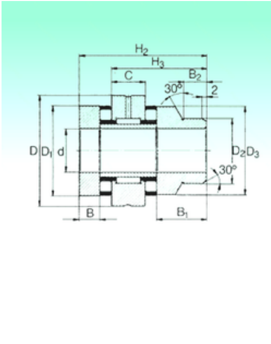
ZARN 90180 L TN Bearing 2D drawings and 3D CAD models
