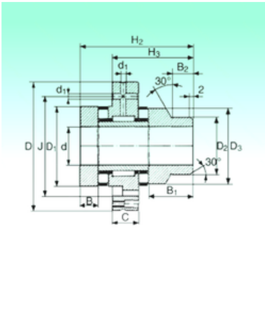
ZARF 45130 L TN Bearing 2D drawings and 3D CAD models
